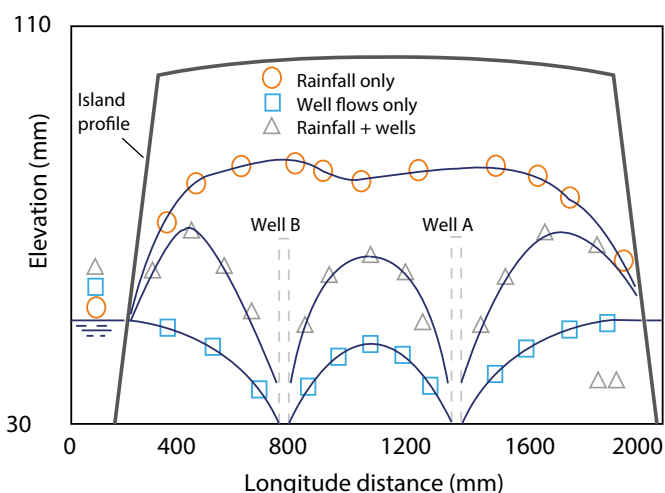
Well abstraction from a circular island
